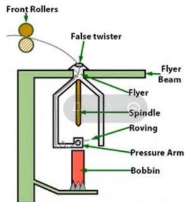
Fig: Twist Insertion on Roving
