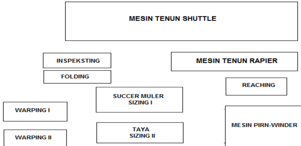
Lampiran 1 Tata Letak Mesin Departemen Weaving
