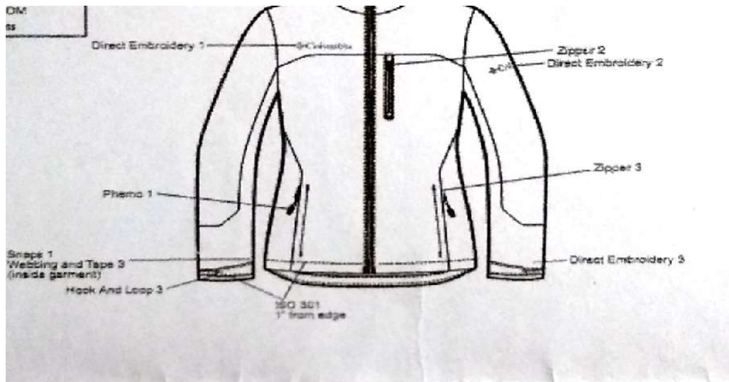
Lampiran 1 Sketsa Front Body Inner Jacket Style XL7263
